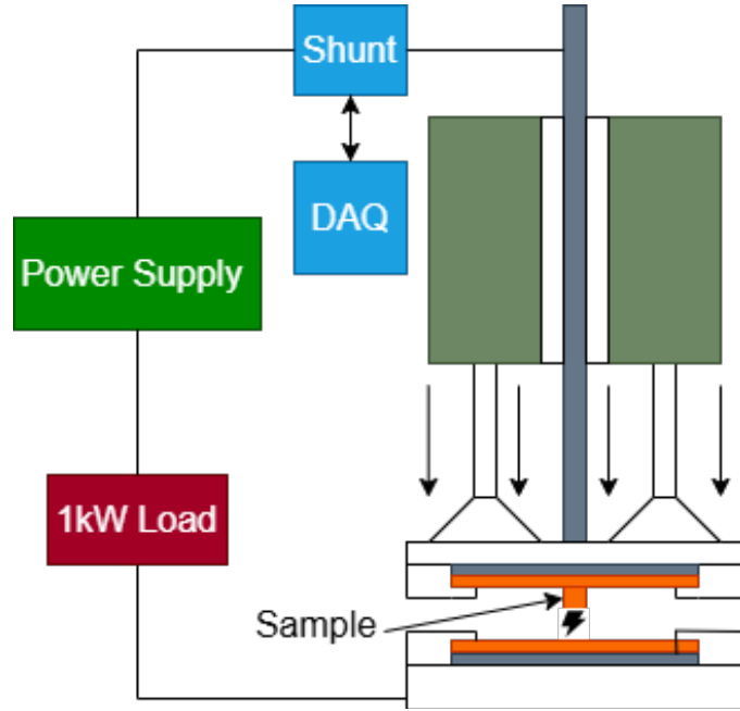
Figure 1. Test Bench diagram
